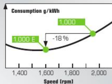
With economy PTO available, the Agrotion can operate within a speed band optimized to minimize energy consumption.
